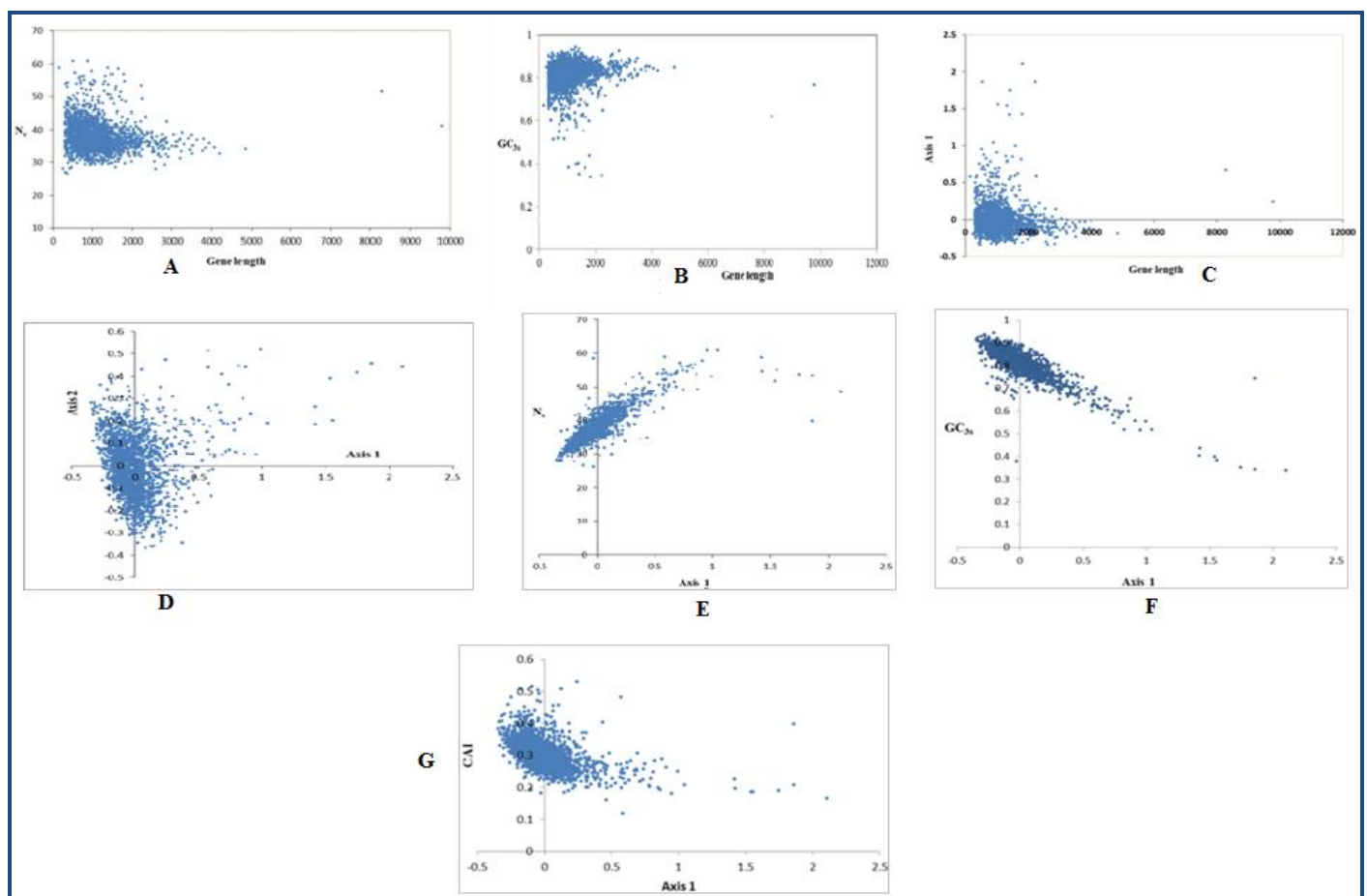
Figure 3: (A) Plot of N c versus gene length; (B) Plot of GC 3s versus gene length; (C) Plot of gene position on axis1 versus gene length; (D) Correspondence analysis of Relative Synonymous Codon Usage values of C. salexigen genes; (E) Scatter plot of gene position on axis 1 and N c values; (F) Scatter plot of gene position on axis 1 and GC 3s values; (G) Scatter plot of gene position on axis 1 and CAI values.
