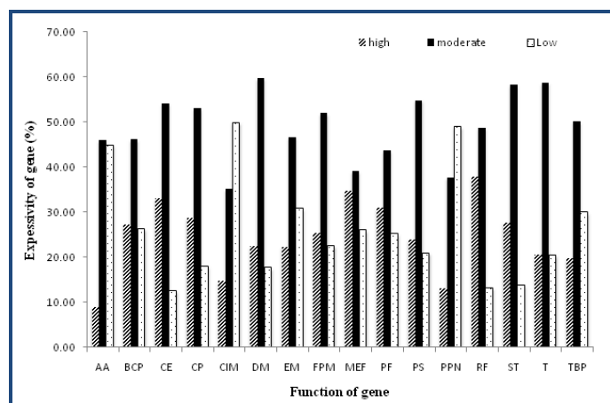
Figure 4: Expression level of functional genes of C. salaxigens on the basis of Axis 1 based on RSCU values. AA = Amino acid biosynthesis; BCP =Biosynthesis of cofactor, Prosthetic groups and carriers; CE =Cell envelope; CP =Cellular processes; CIM =Central intermediary metabolism; DM =DNA metabolism; EM =Energy metabolism; FPM =Fatty acid & phospholipid metabolism; MEF =Mobile & extrachromosomal element functions; PF =Protein fate; PS =Protein synthesis; PPN =Purines, pyrimidines, nucleosides & nucleotides; RF =Regulatory functions; ST =Signal transduction; T =Transcription; TBP =Transport & binding protein
